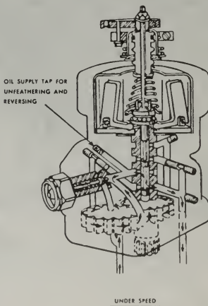
FIGURE 7-16. Woodward Governor X210,000 Series
